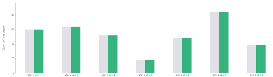
Obr. 2: Velocity report
