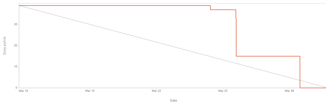
Obr. 1: Burndown chart
