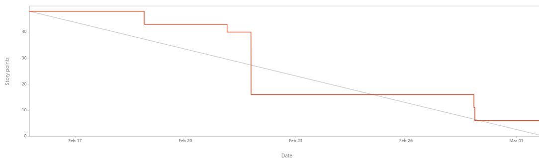
Obr. 1: Burndown chart
