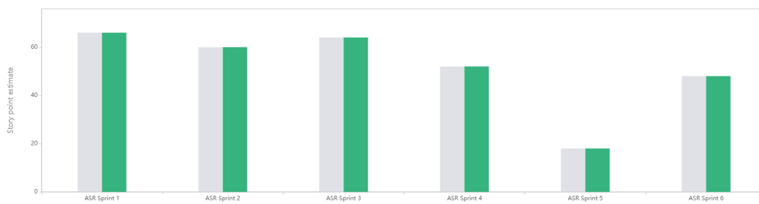
Obr. 2: Velocity report
