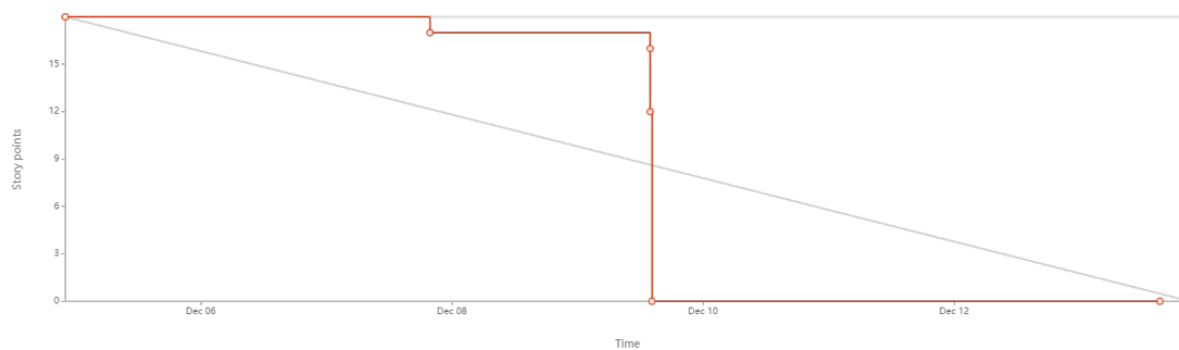
Obr. 1: Burndown chart
