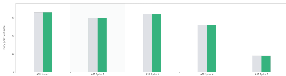
Obr. 2: Velocity report
