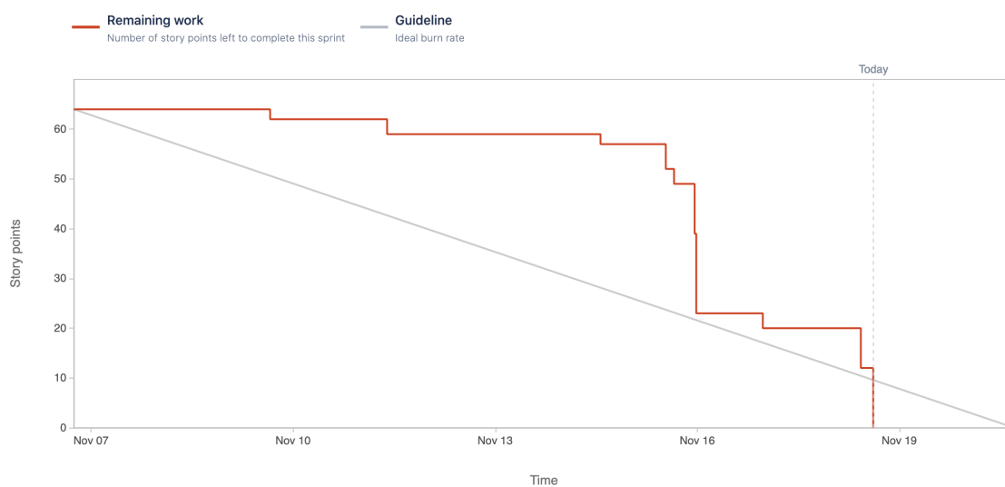
Obr. 1: Burndown chart
