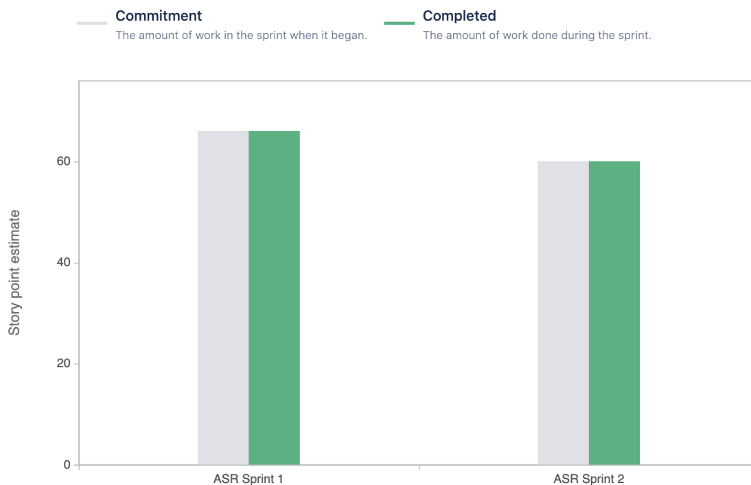
Obr. 2: Velocity report
