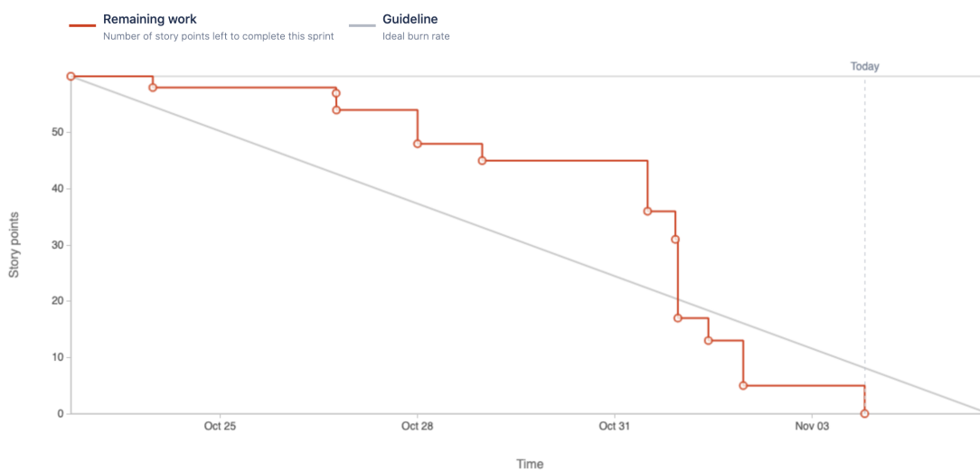
Obr. 1: Burndown chart
