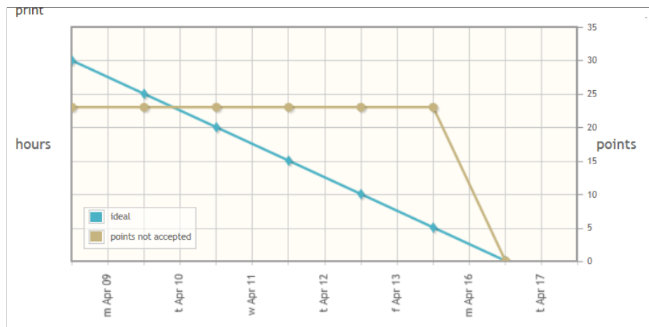
Obr. 12: Burndown chart pre šprint Tesing
