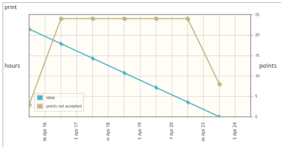
Obr. 13: Burndown chart pre šprint After-Test
