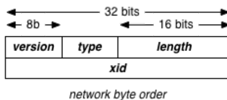
Obr. 4. - OpenFlow hlavička
