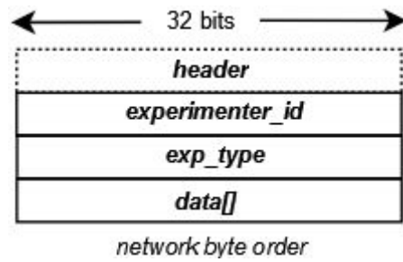
Obr. 5. - Experimenter hlavička
