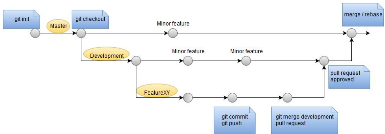
Obr. 1: Git workflow
