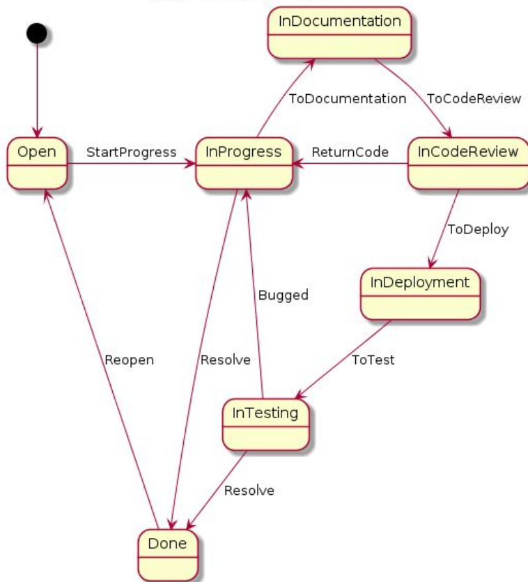
JIRA Workflow - IndoorNav
