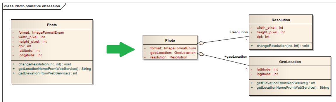
Obr. F.2: Photo primitive obsession
