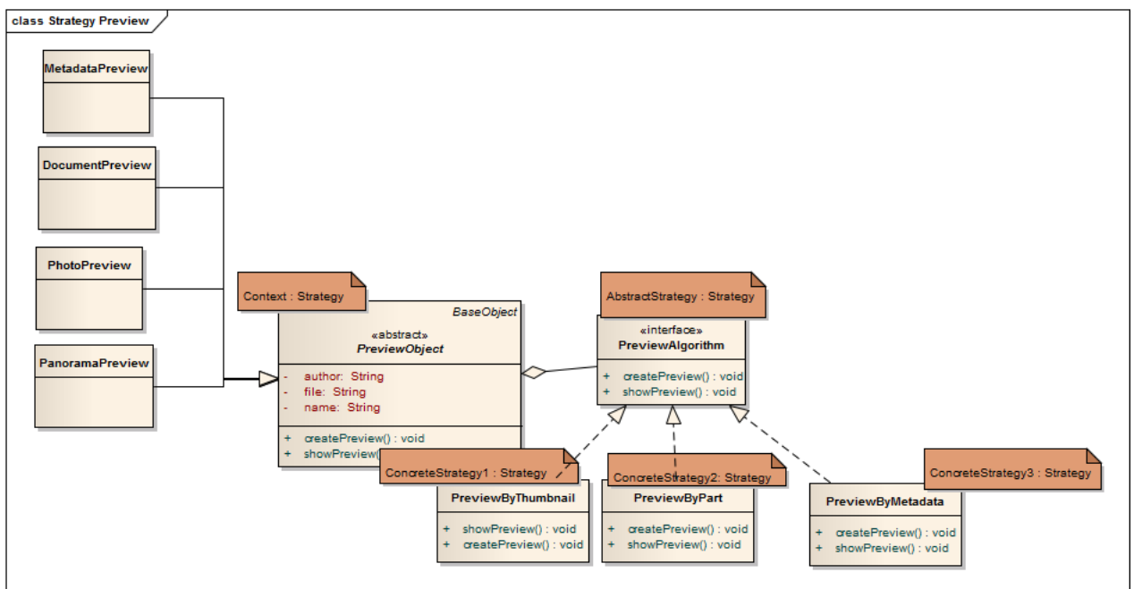
Obr. E.4: Strategy 2
