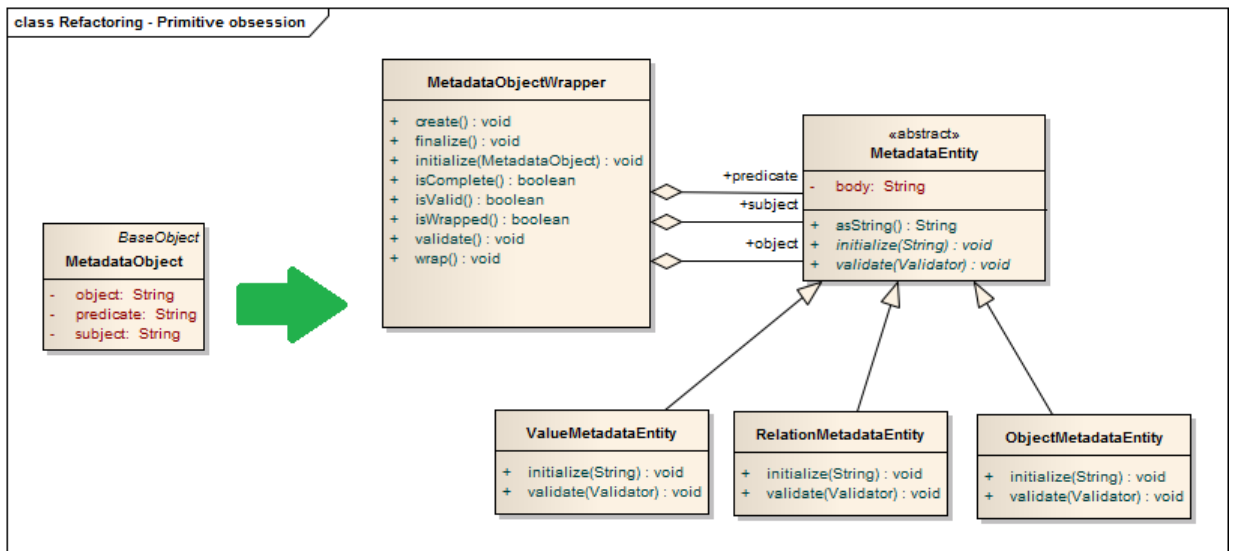
Obr. F.1: Refactoring - Primitive obsession
