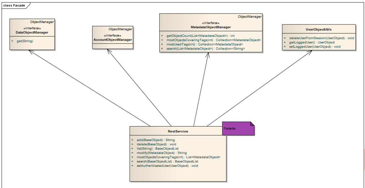
Obr. E.6: Facade
