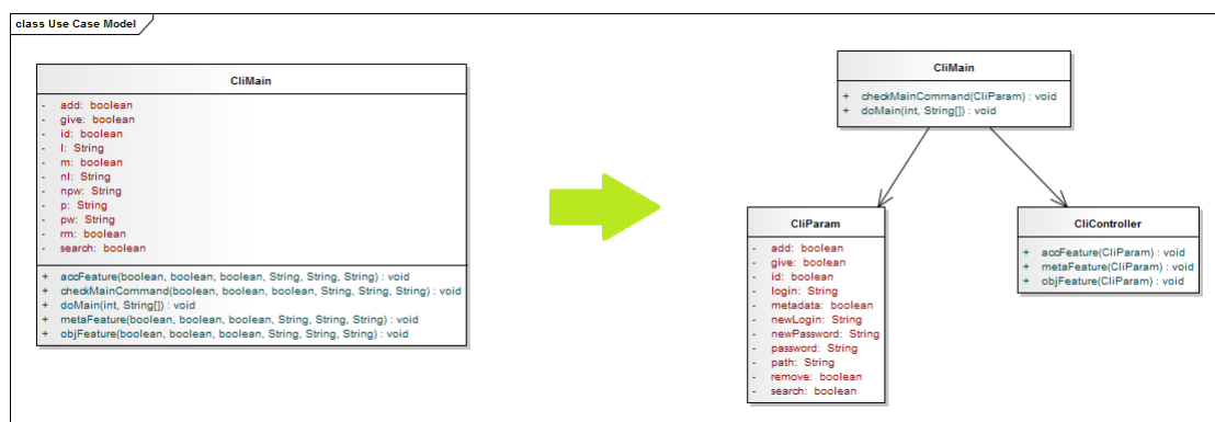
Obr. F.4: Refactoring - Large Class MetadataManagerImpl
