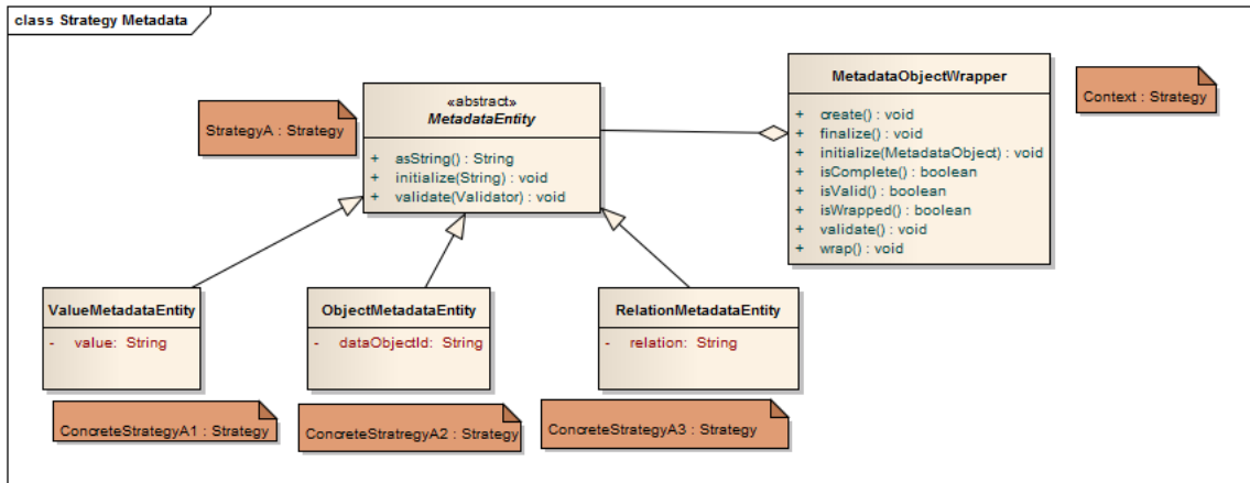
Obr. E.3: Strategy 1
