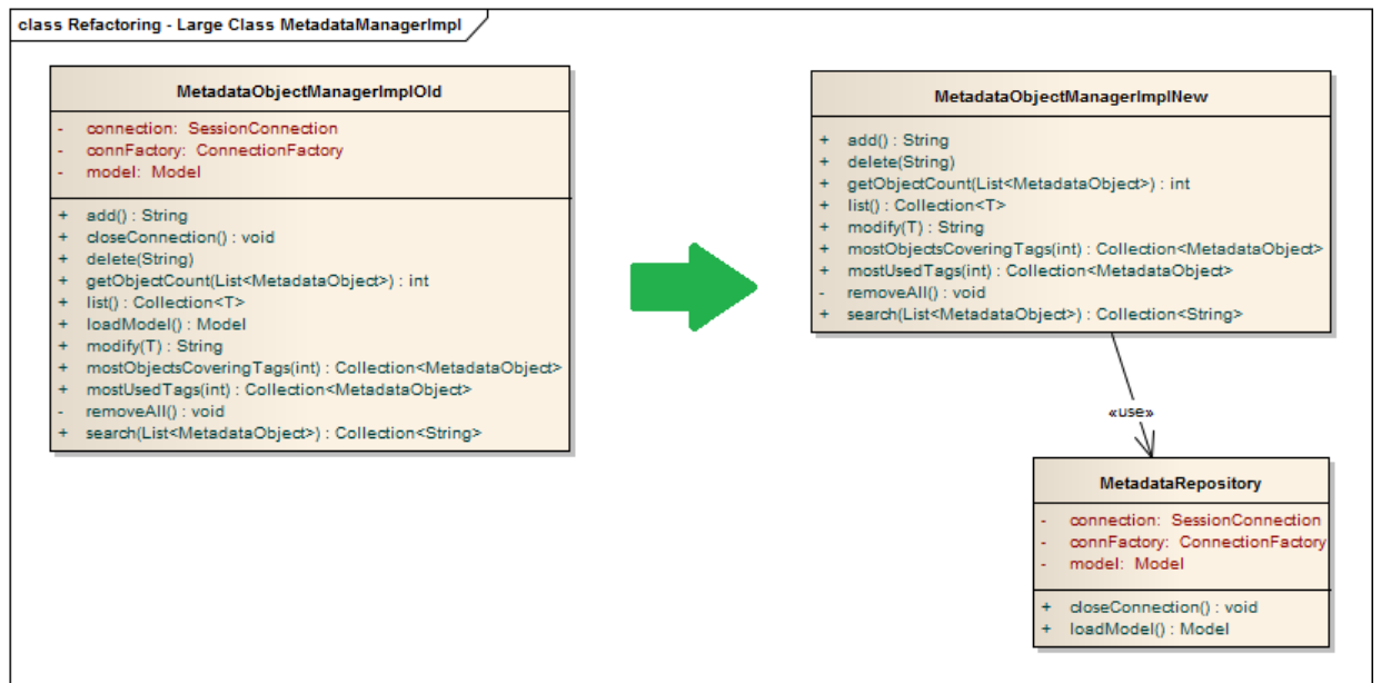
Obr. F.3: Refactoring - Large Class MetadataManagerImpl
