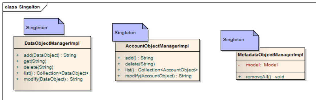
Obr. E.8: Singleton
