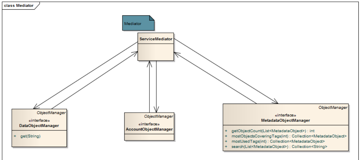
Obr. E.7: Mediator
